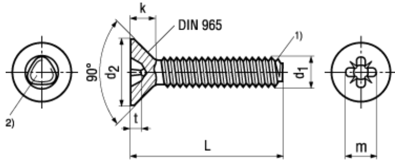
1) Tapered thread end max. 4P 2) Trilobular
